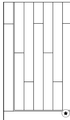
Random straight laid plank with single plank and strip perimeter. Design ref: 501
