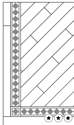
45° Straight laid plank with design border and single plank perimeter Design ref: 519
