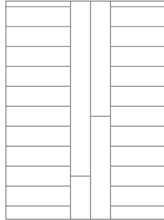
Double plank tramline Design ref: 215
