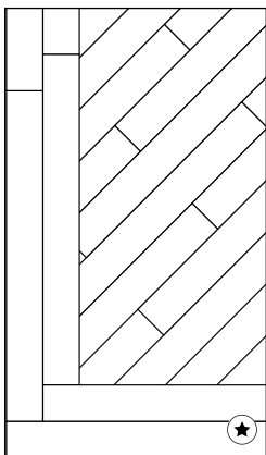
45° Straight laid plank with double plank perimeter. Design ref: 504
