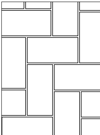
Stone herringbone using rectangular tiles and strip. Design ref: 429
