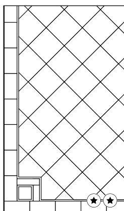
Square tile laid 45° with half tile & strip perimeter & inset corner tile Design ref: 530
